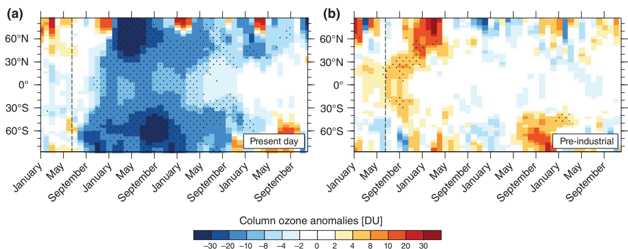
FIGURE 6 | Zonal mean column ozone changes [DU] by heterogeneous chemical reactions in an ensemble of atmosphere–ocean–chemistry climate simulations for a 4× Pinatubo eruption in a present day (left) and preindustrial (right) atmosphere (modified from Muthers et al. 103 ). Vertical dashed line indicates the beginning of the eruption. Significant anomalies with respect to an ensemble of control simulations are shown by stippling.
